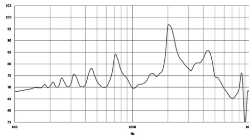
Frequency Response
